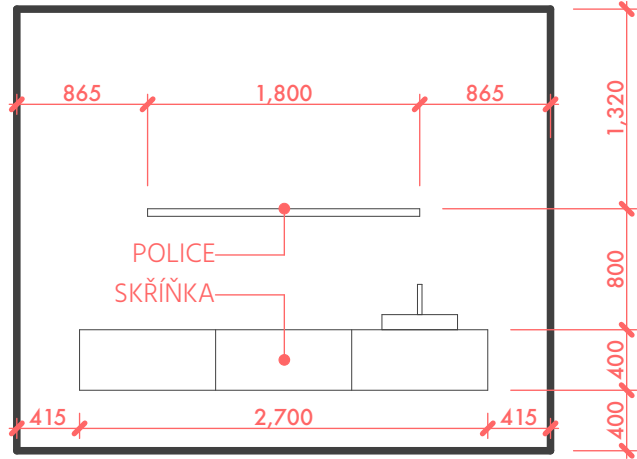
S.65/B + S.66/B | MASÉRNA
